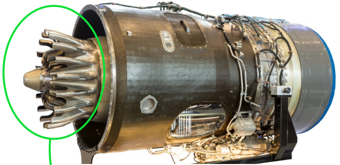
Turbine Exhaust Case Including Additive Manufacturing component
